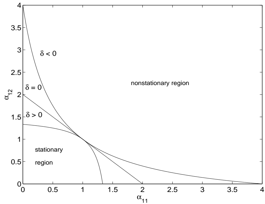
Figure 1: Stationarity regions for the univariate two-regime Markov-switching ARCH(1) processes characterized by the transition matrices given in (33).
