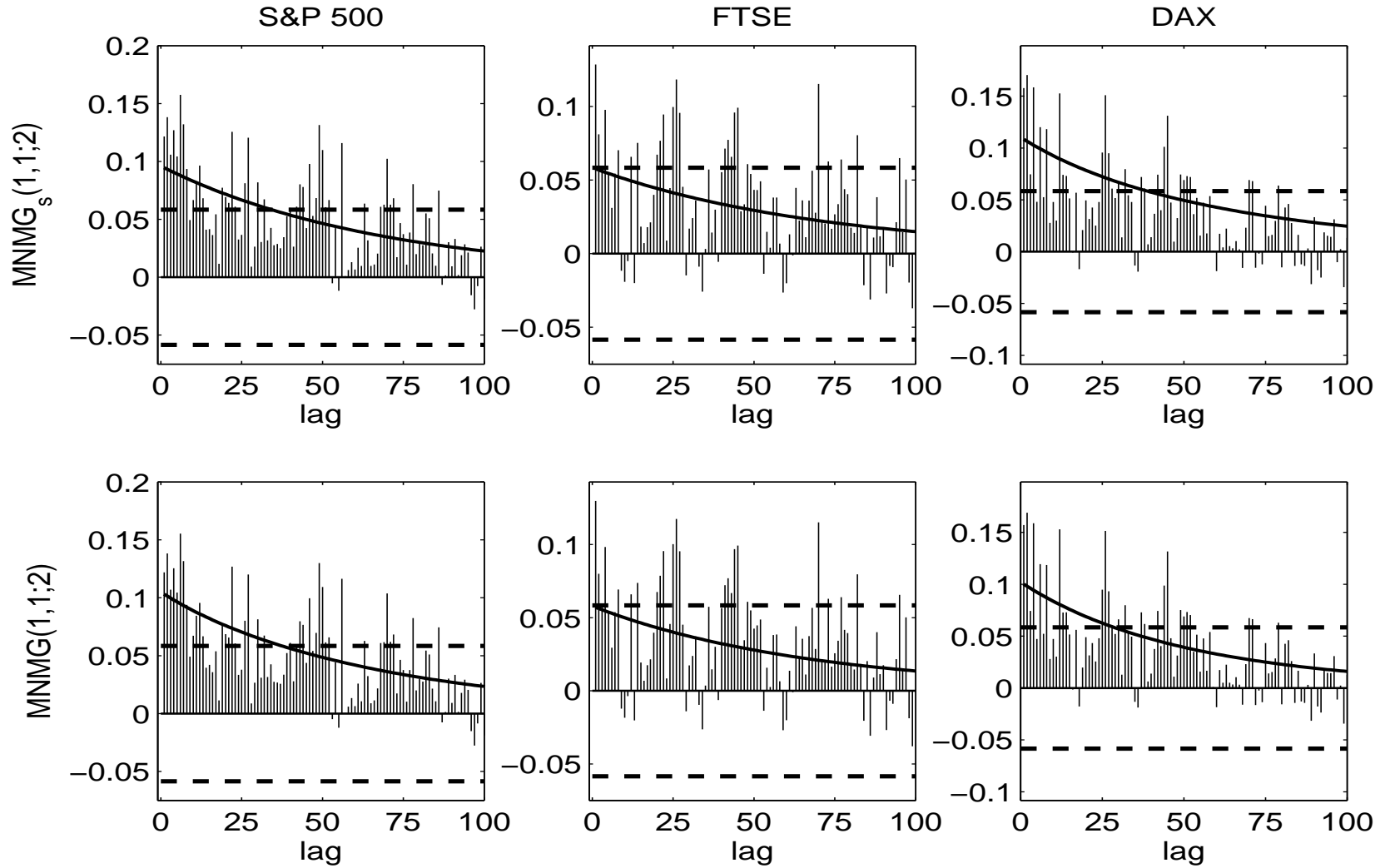
Figure 3: Shown are, from left to right, the sample autocorrelations of the squared returns of the S&P500, the FTSE, and the DAX, along with their theoretical counterparts as implied by, from top to bottom, the fitted MNMG_s(1,1) and MNMG(1,1;2) models. The theoretical autocorrelation function is defined in (38). Dashed lines represent approximate 95% one-at-a-time confidence intervals.
