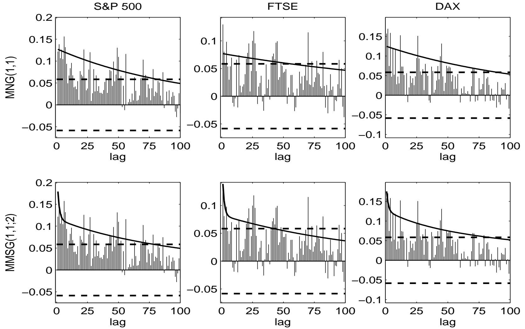
Figure 2: Shown are, from left to right, the sample autocorrelations of the squared returns of the S&P500, the FTSE, and the DAX, along with their theoretical counterparts as implied by, from top to bottom, the fitted MNG(1,1) and MMSG(1,1;2) models. The theoretical autocorrelation function is defined in (38). Dashed lines represent approximate 95% one-at-a-time confidence intervals.
